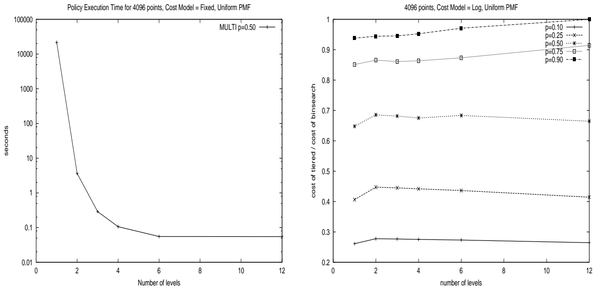
(a) Execution cost of computing tiered search policy (b) Performance of hierarchical policy relative to binary search.
